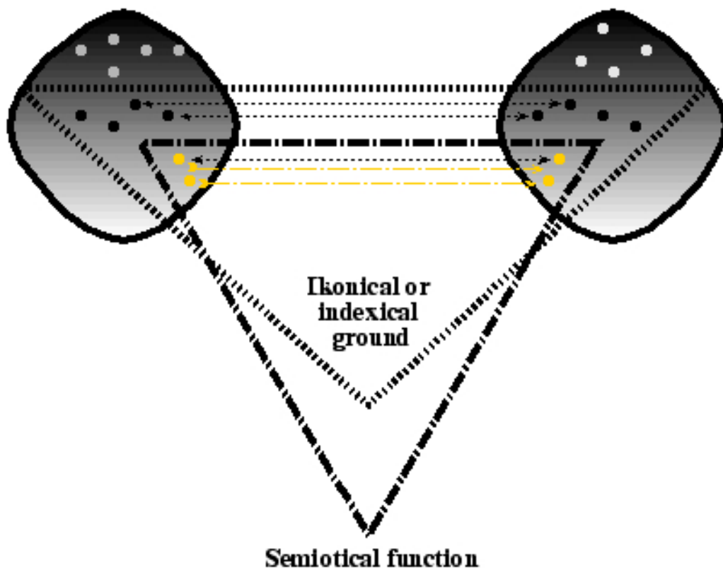
Fig. 3. The sign as a mapping between different spaces
